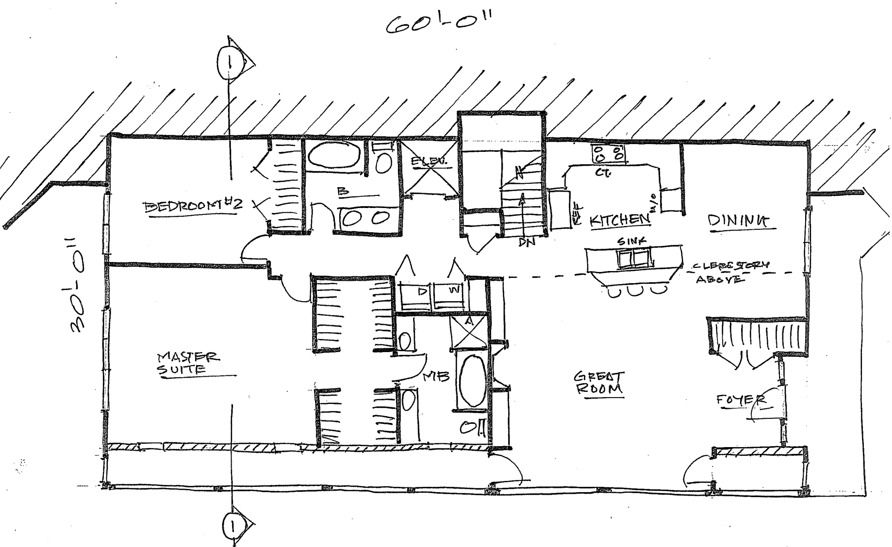
A MAIN FLOOR PLAN @ 1/8" = 1'-0"
