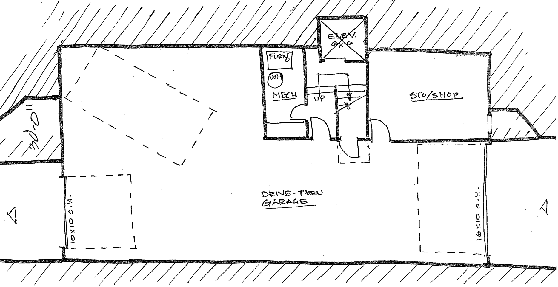
LOWER FLOOR PLAN @ 1/8" = 1'-0"
