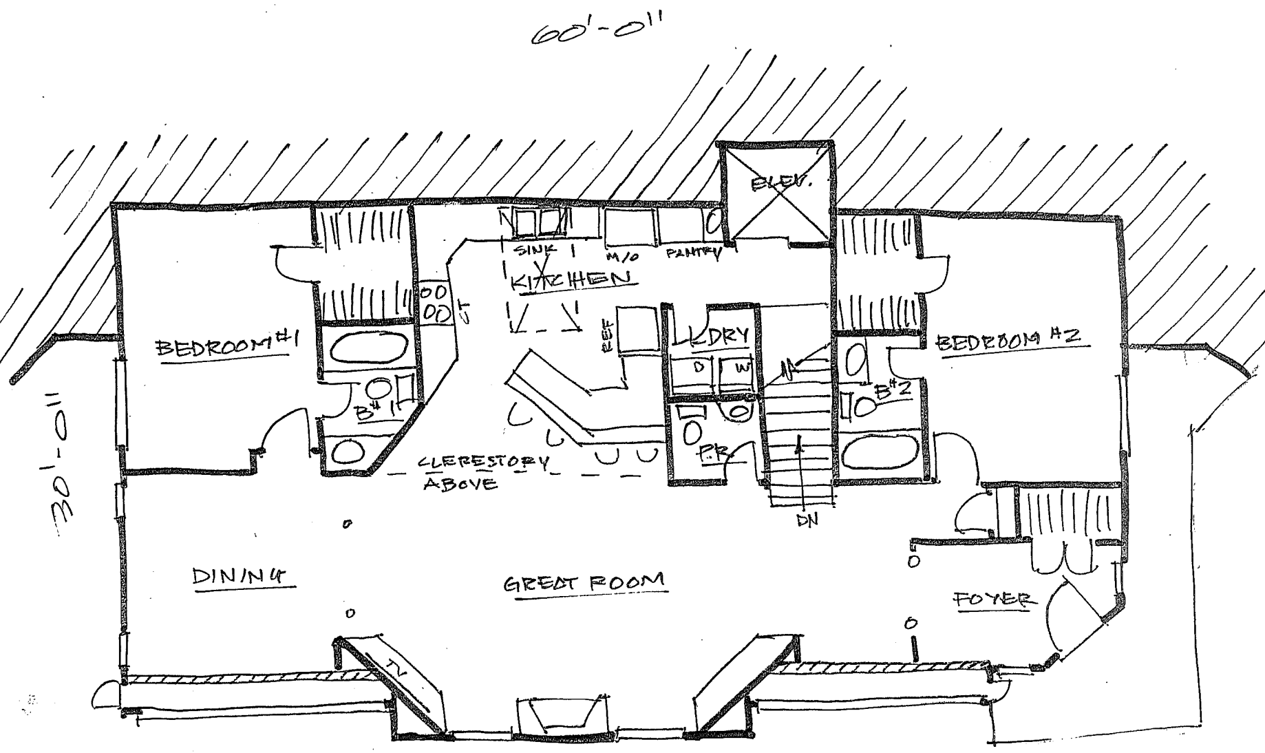
B MAIN FLOOR PLAN @ 1/8" = 1'-0" ▲ NORTH
