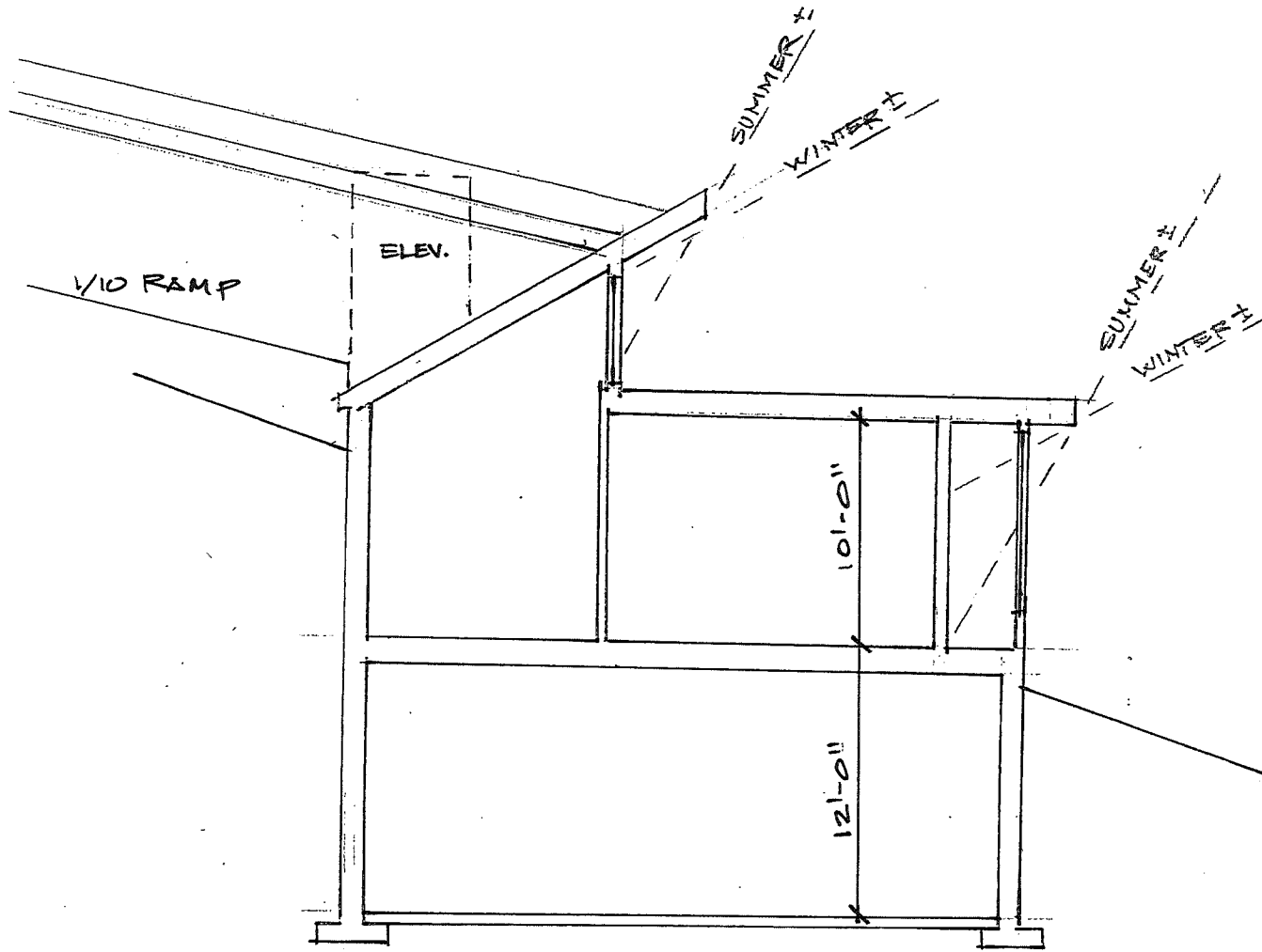
SECTION THRU BEDROOMS @ 1/8" = 1'-0"
